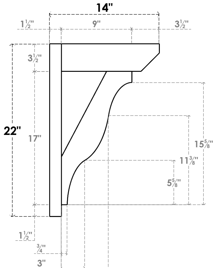
SIDE PROFILE
